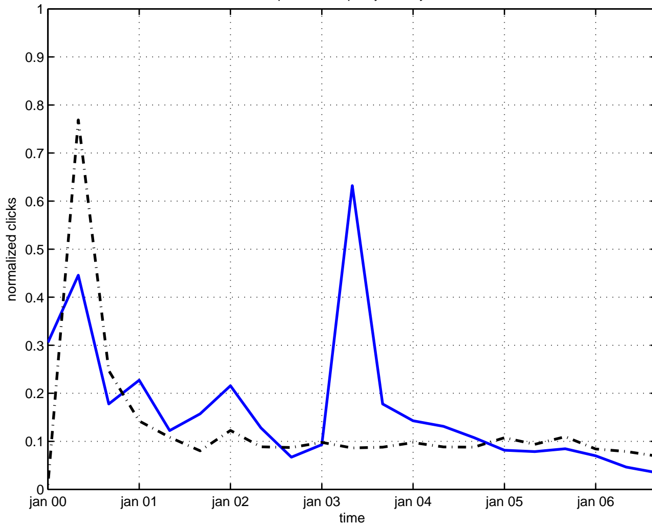
potential supersymmetry
