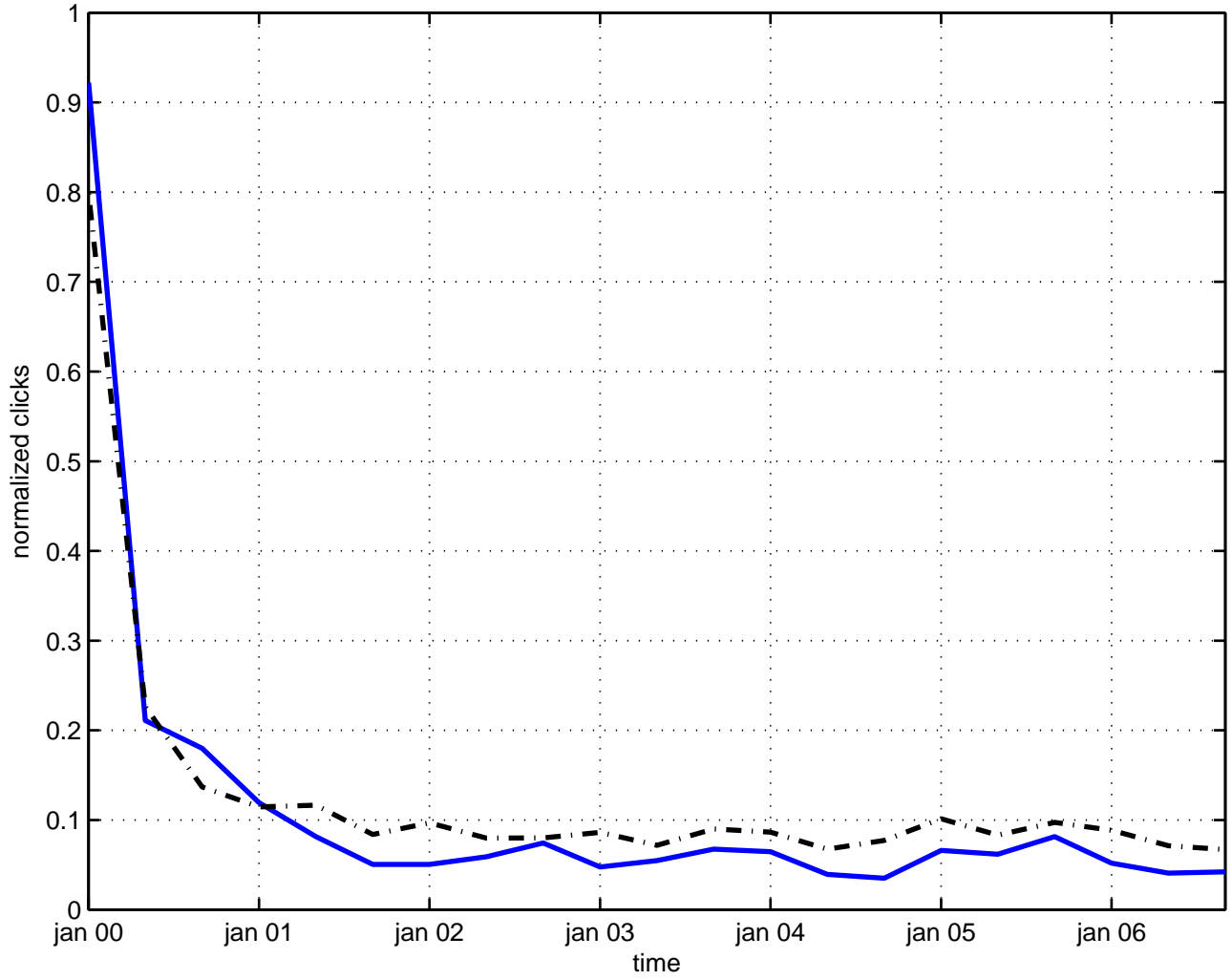
potential supergravity
