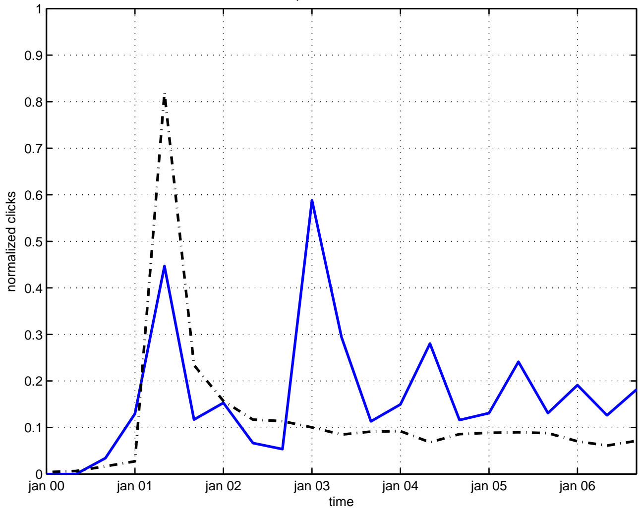
potential radion
