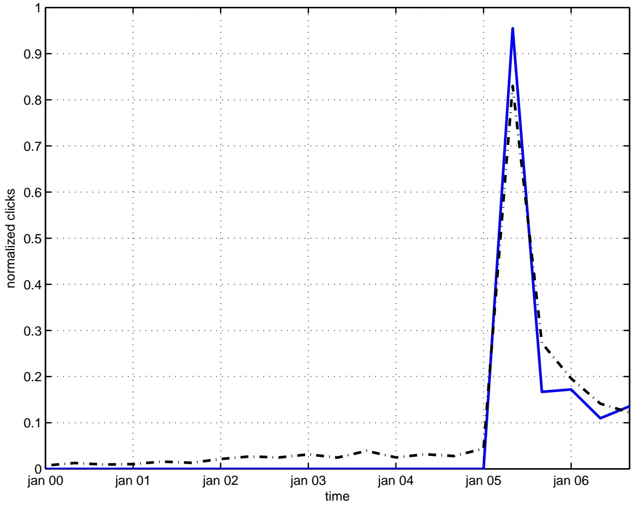
potential quantum gravity
