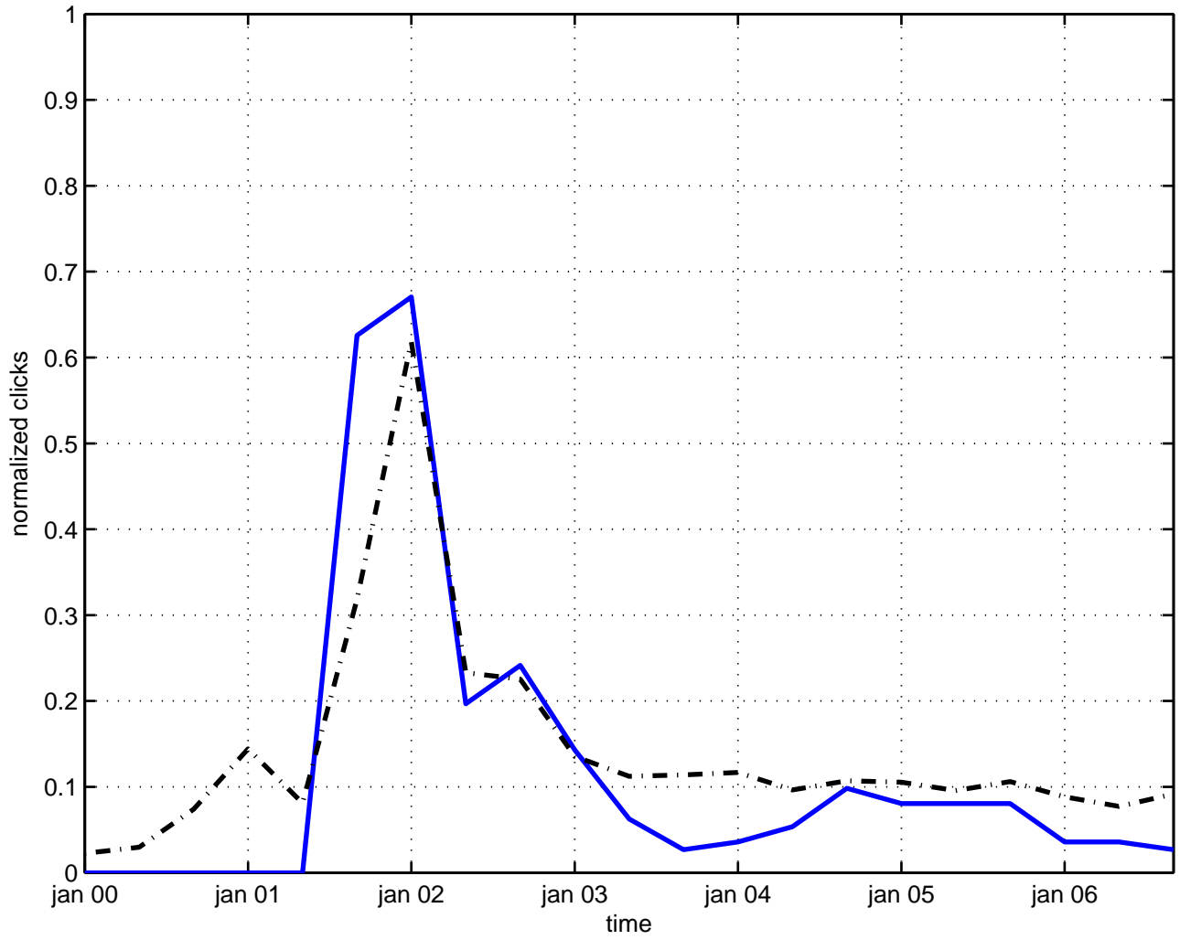
potential monopole
