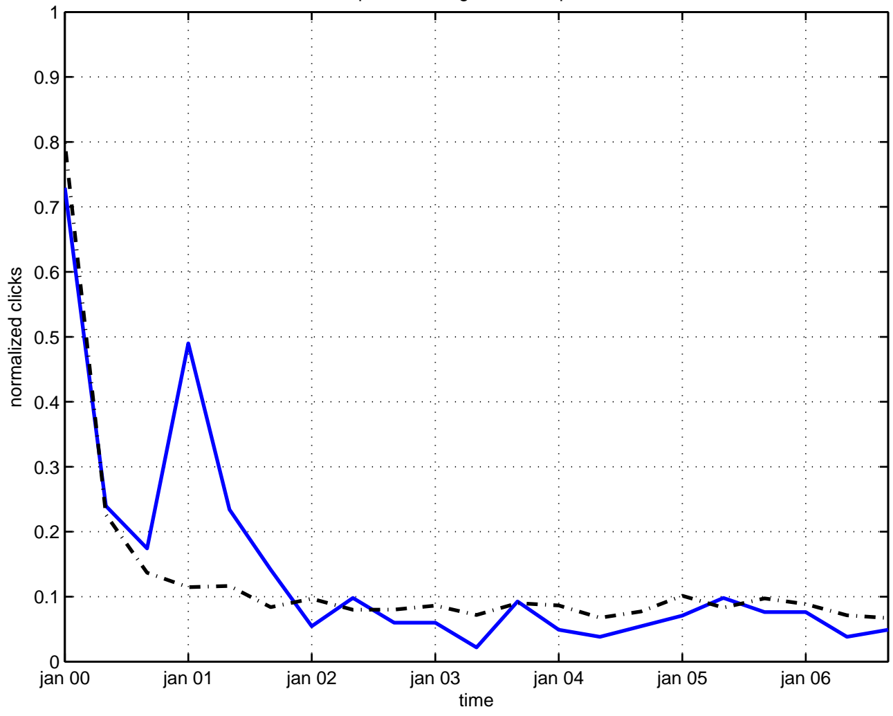
potential magnetic monopole
