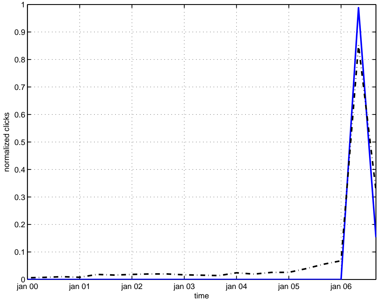
potential instanton
