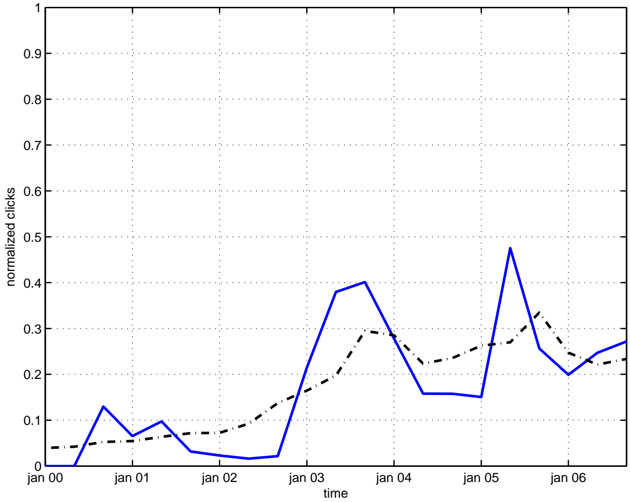
potential inflaton
