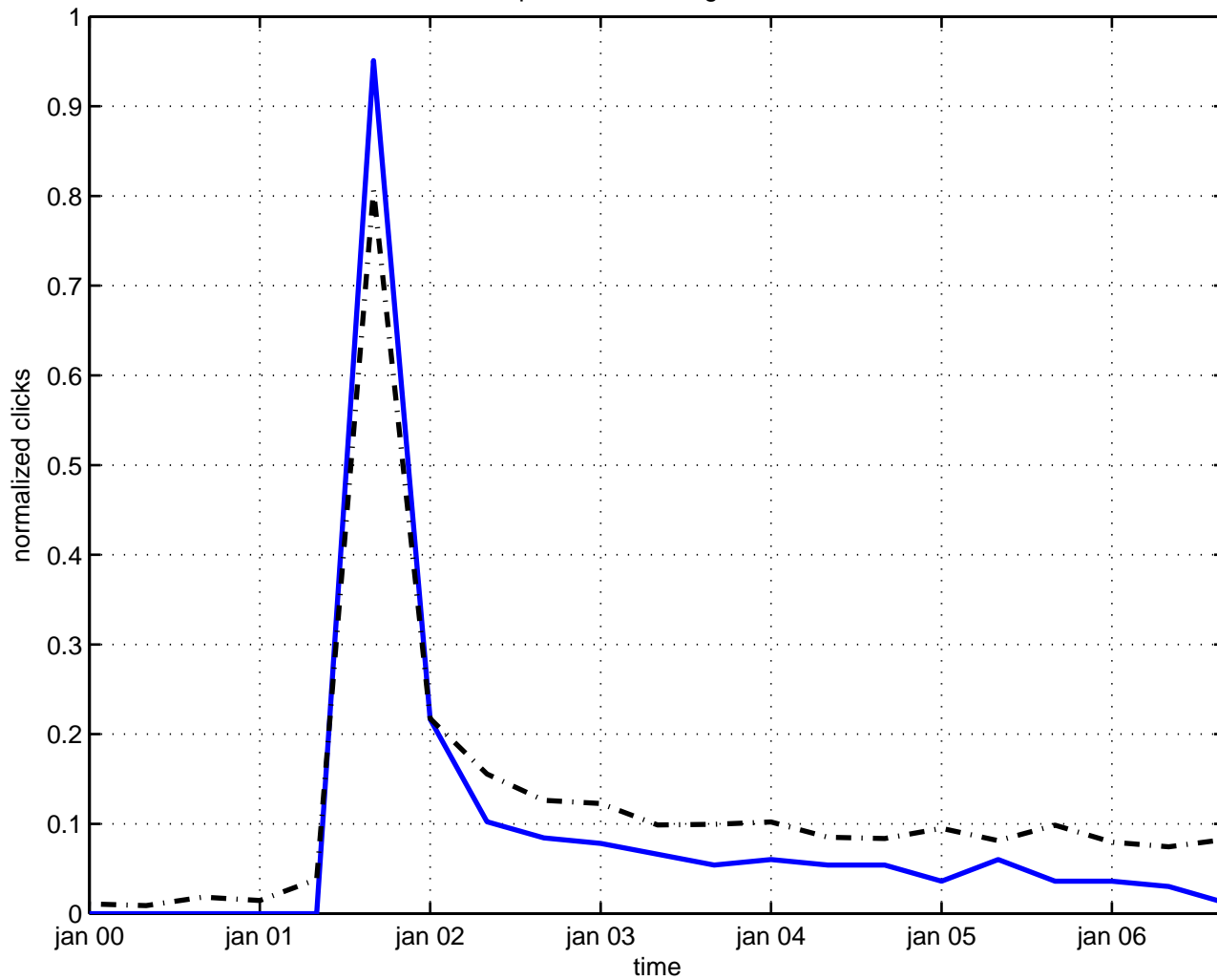
polarization string model
