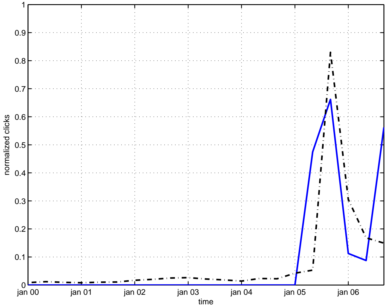
polarization gluon
