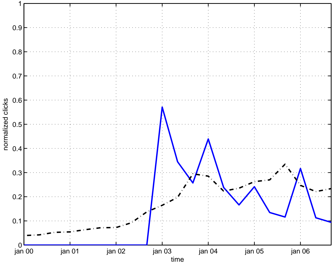
polarization cosmic radiation
