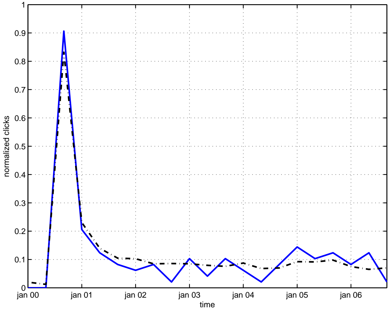
polarizability particle
