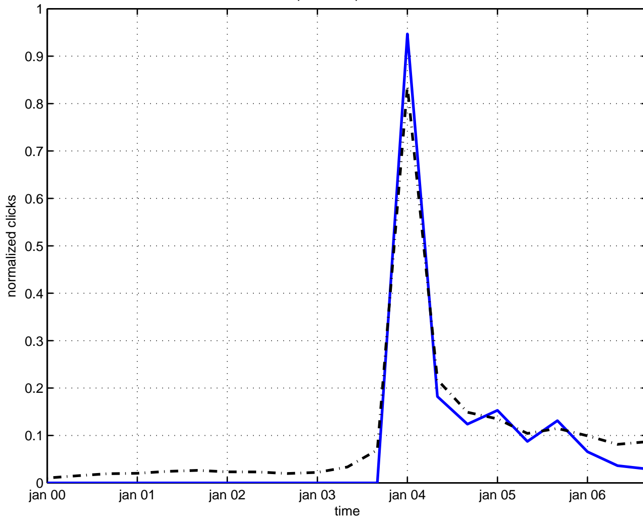
poisson operator
