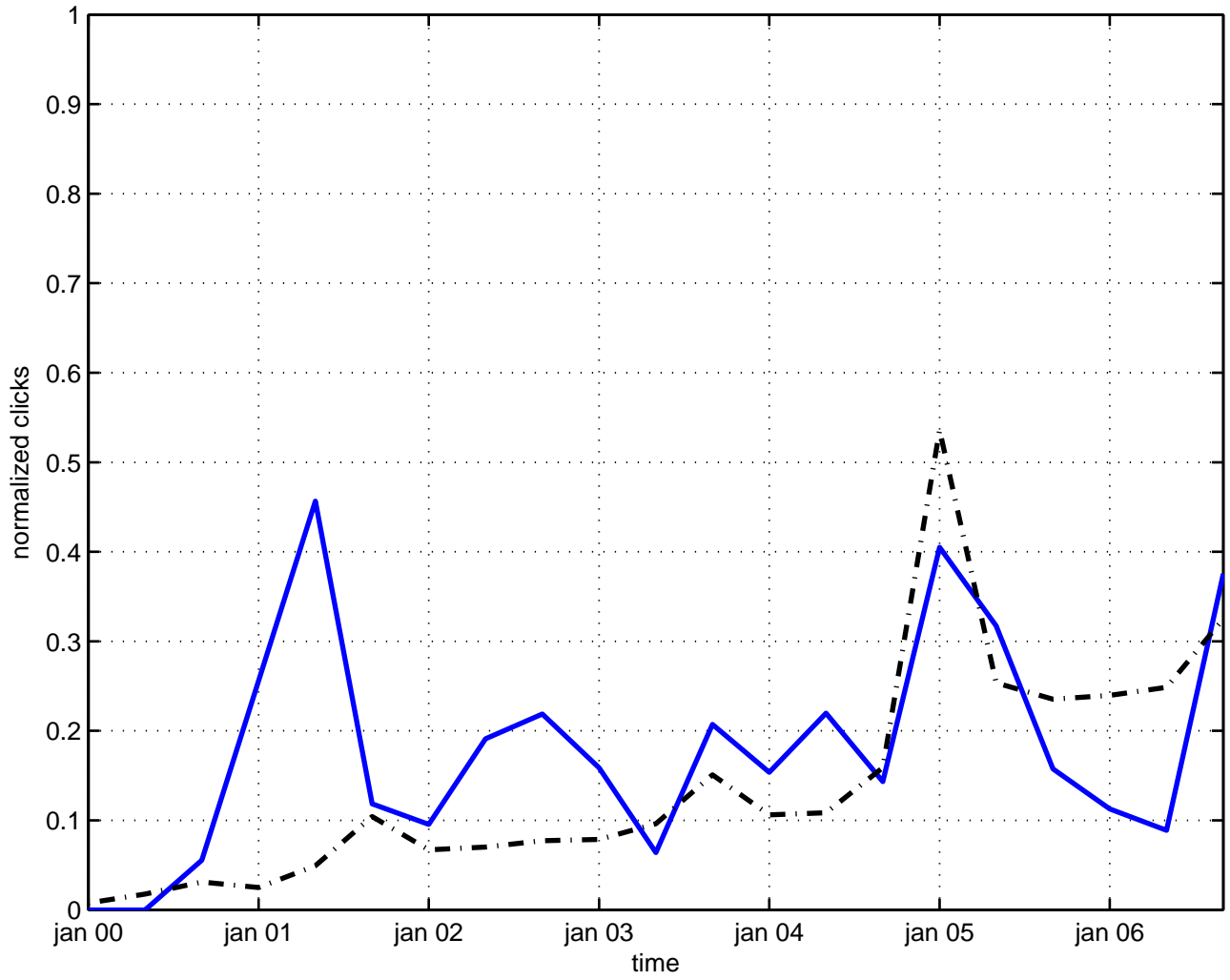
poisson algebra
