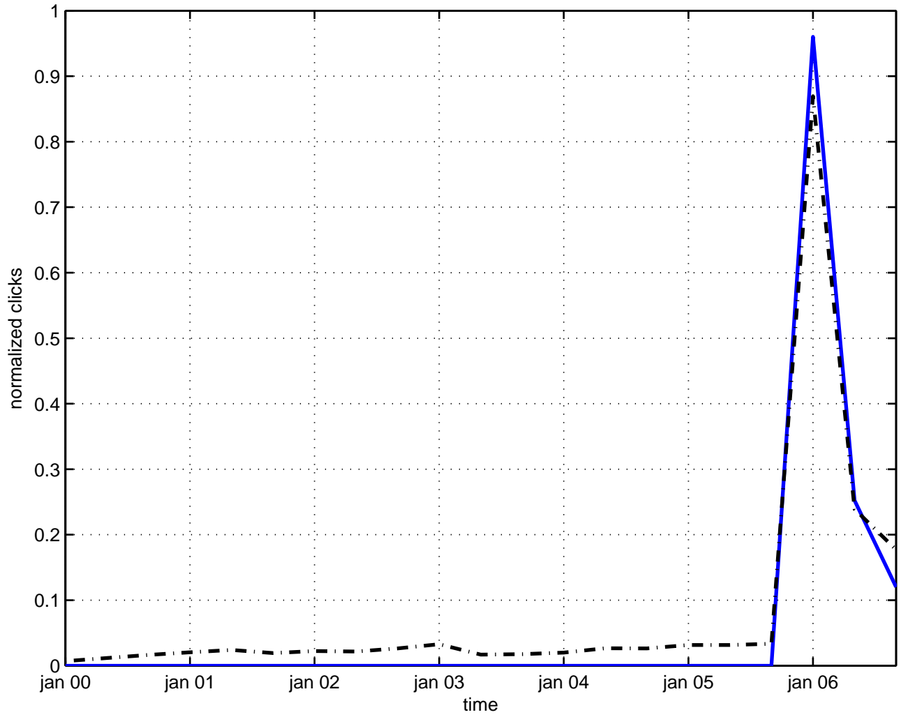
poincare violation
