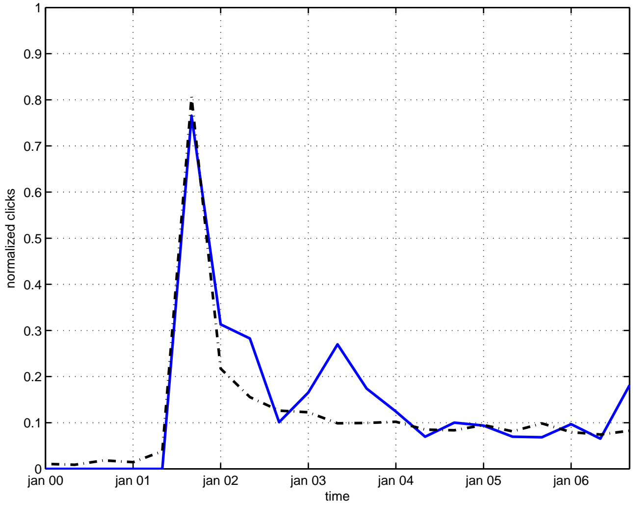
poincare symmetry breaking
