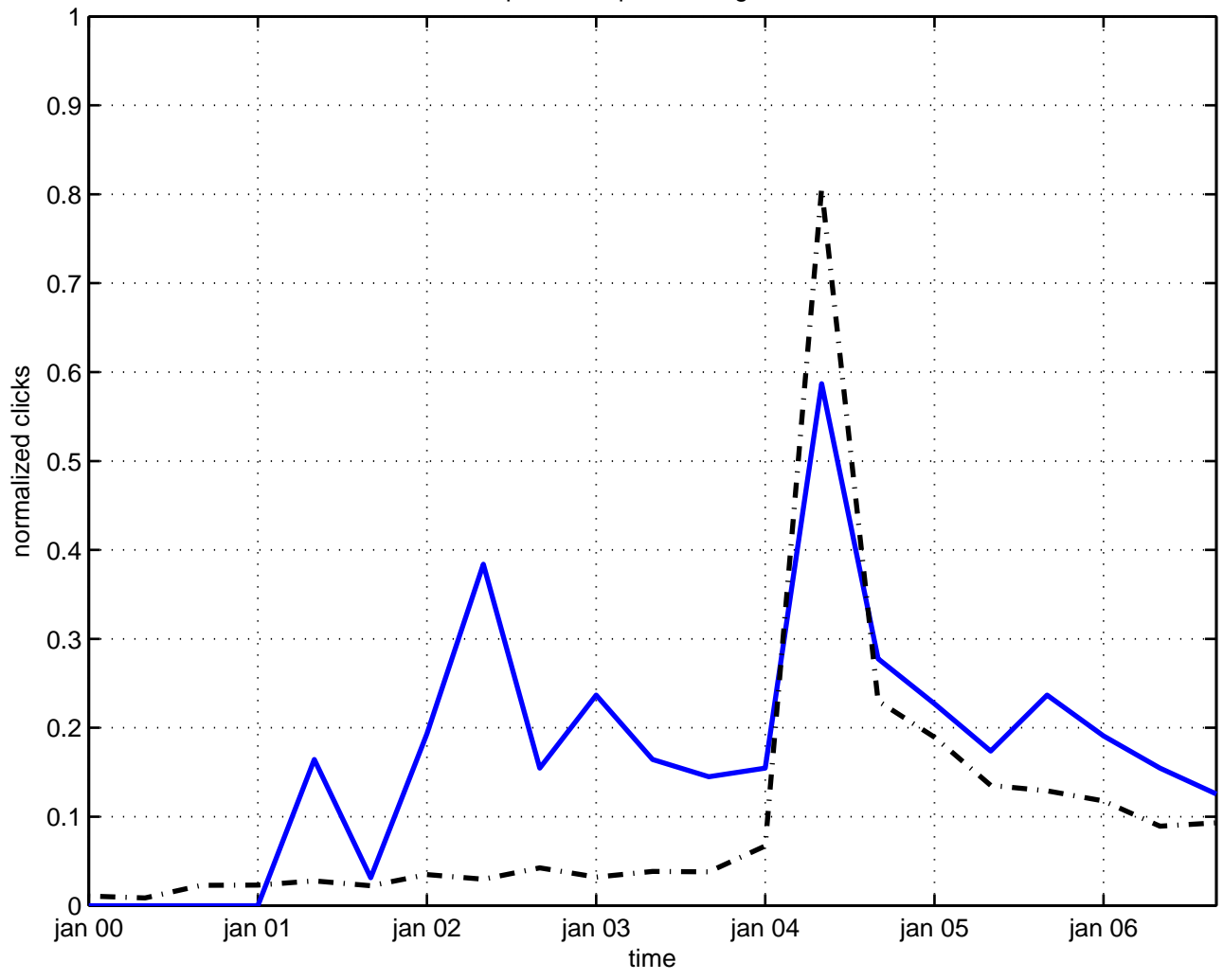
poincare quantum algebra
