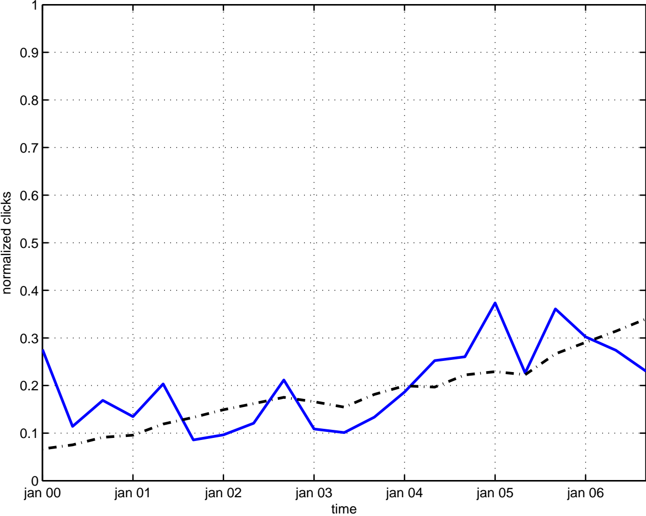
poincare invariance
