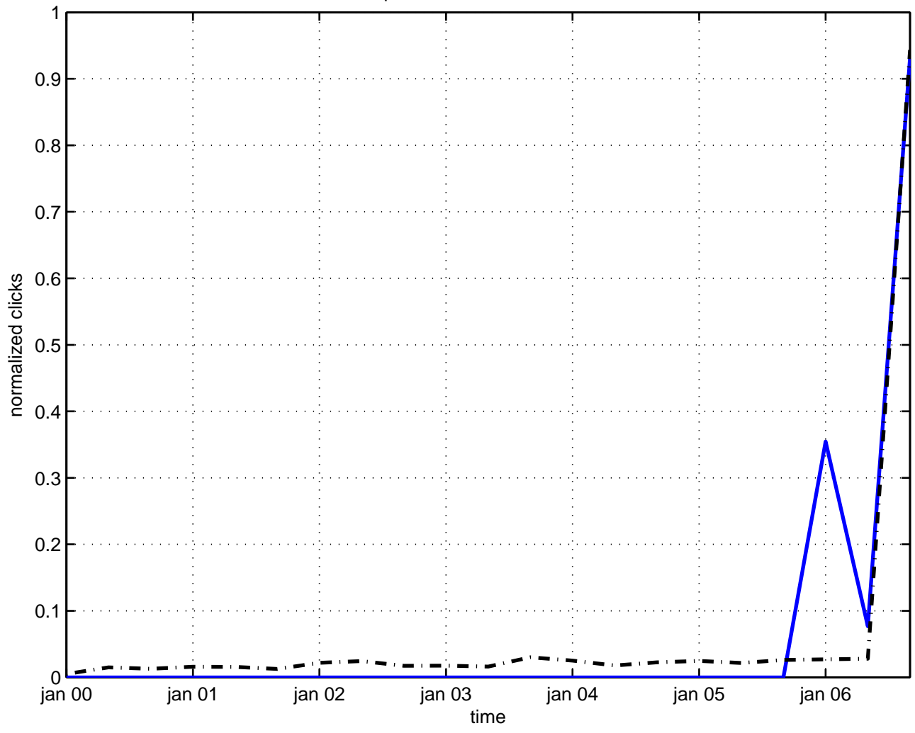
plane wave matrix model
