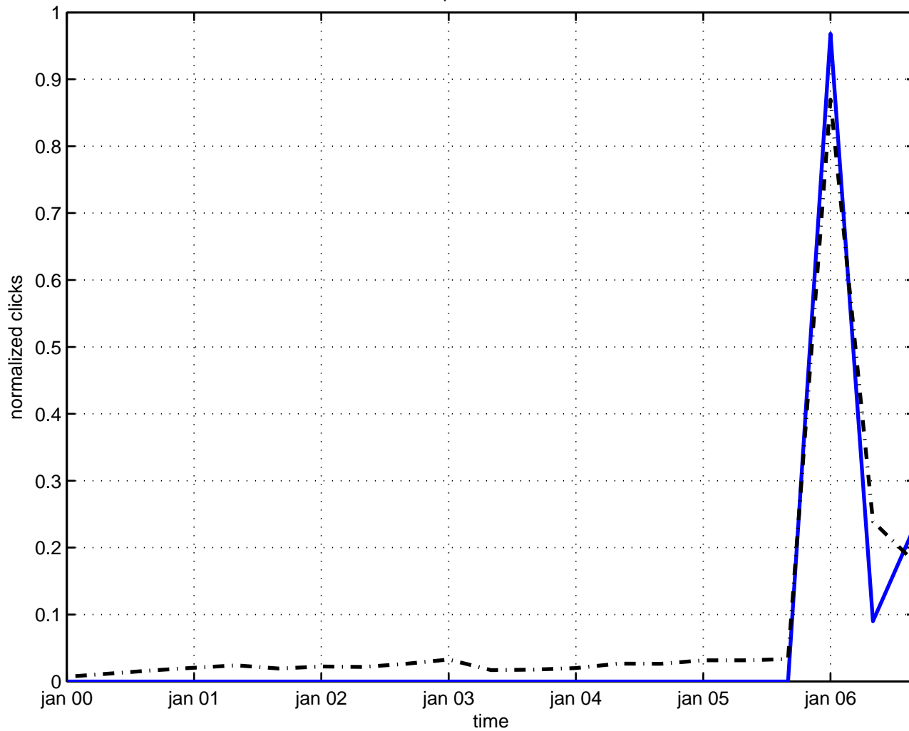
planck time
