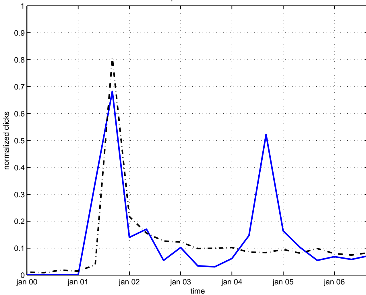
planck constant
