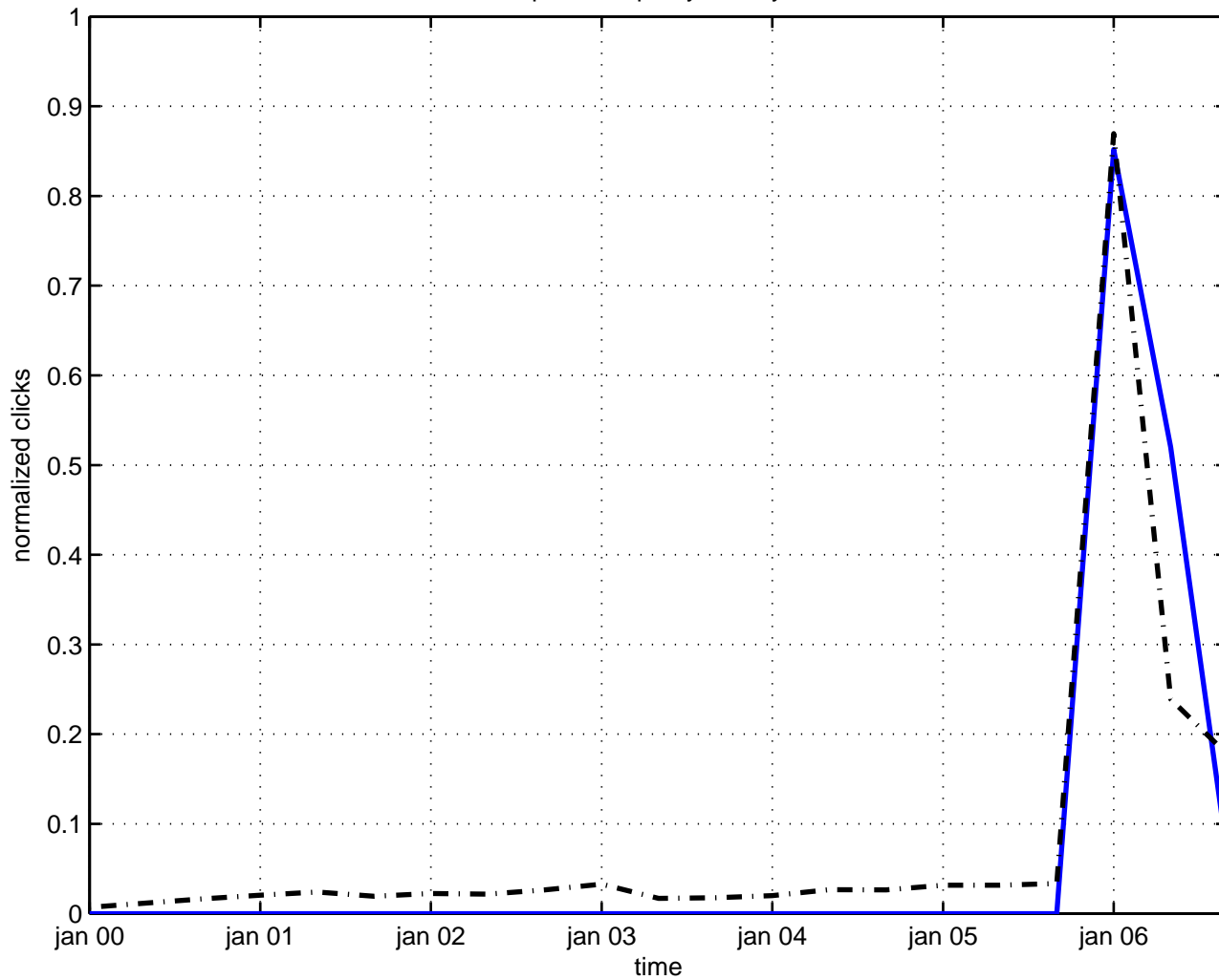
planar supersymmetry
