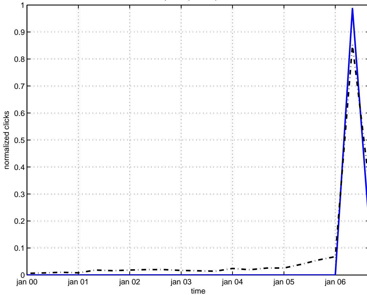
planar phase space
