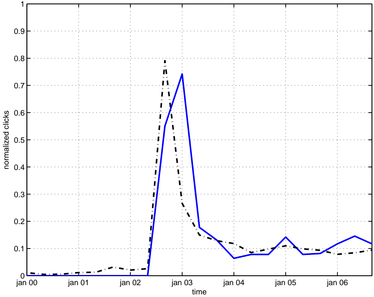
photoproduction black hole
