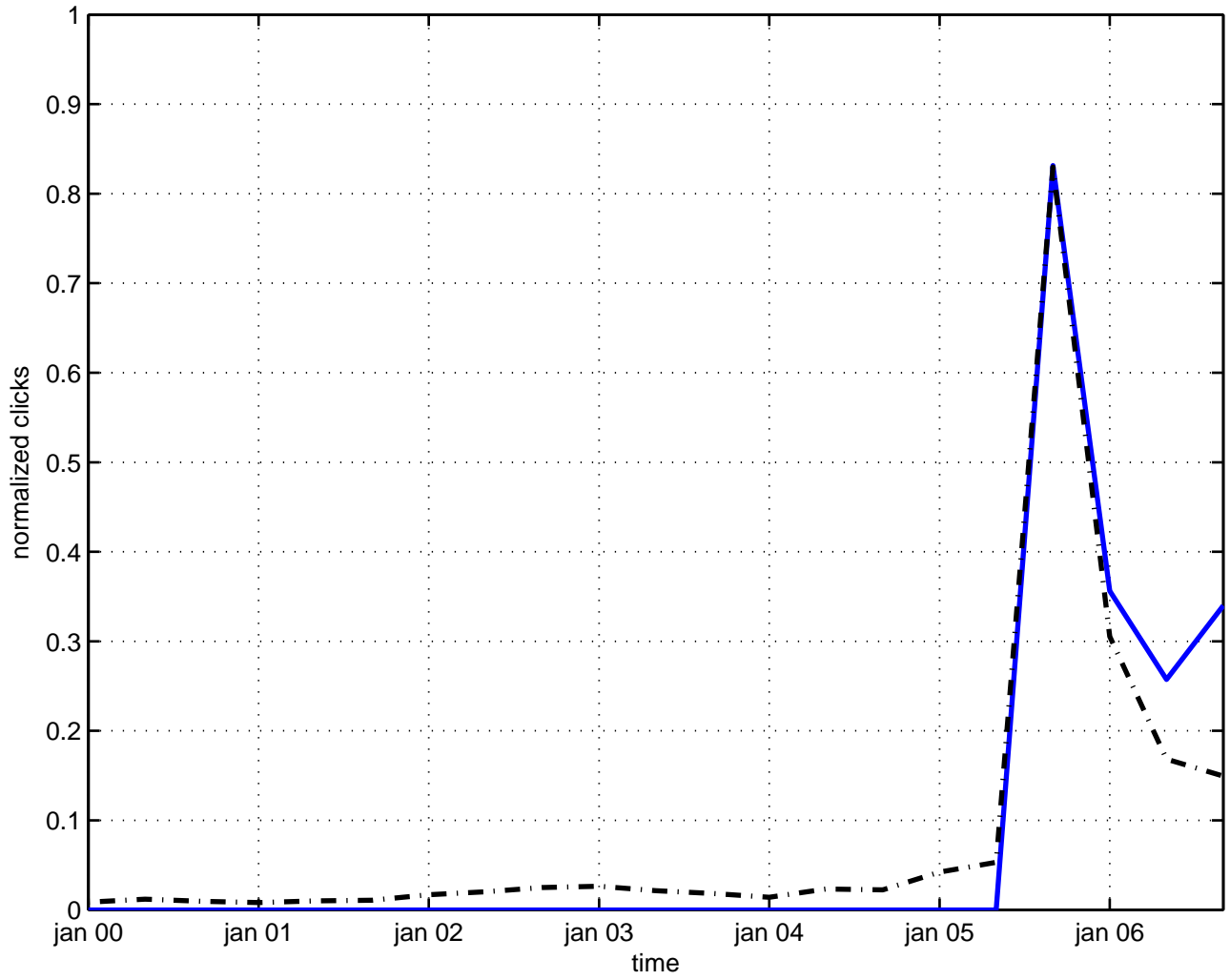
photon pair production
