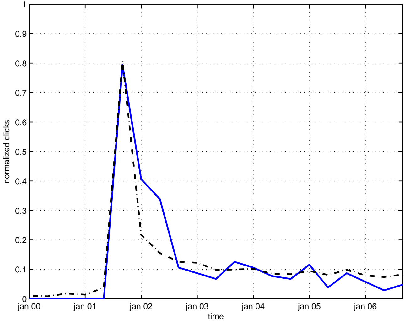
photon p --> delta(1232)
