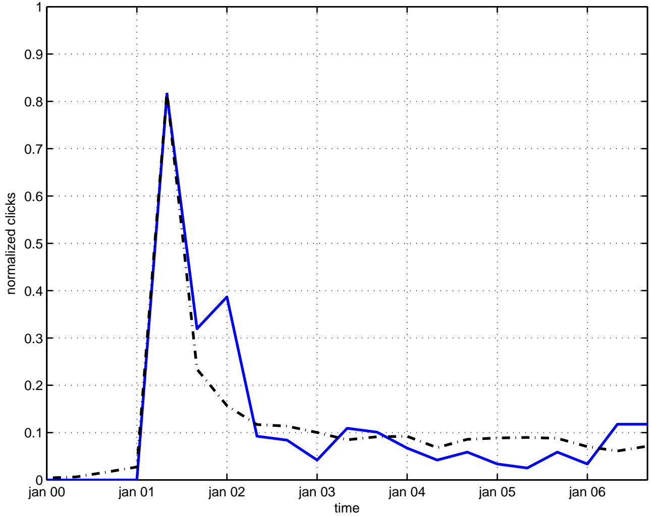
photon axion scattering
