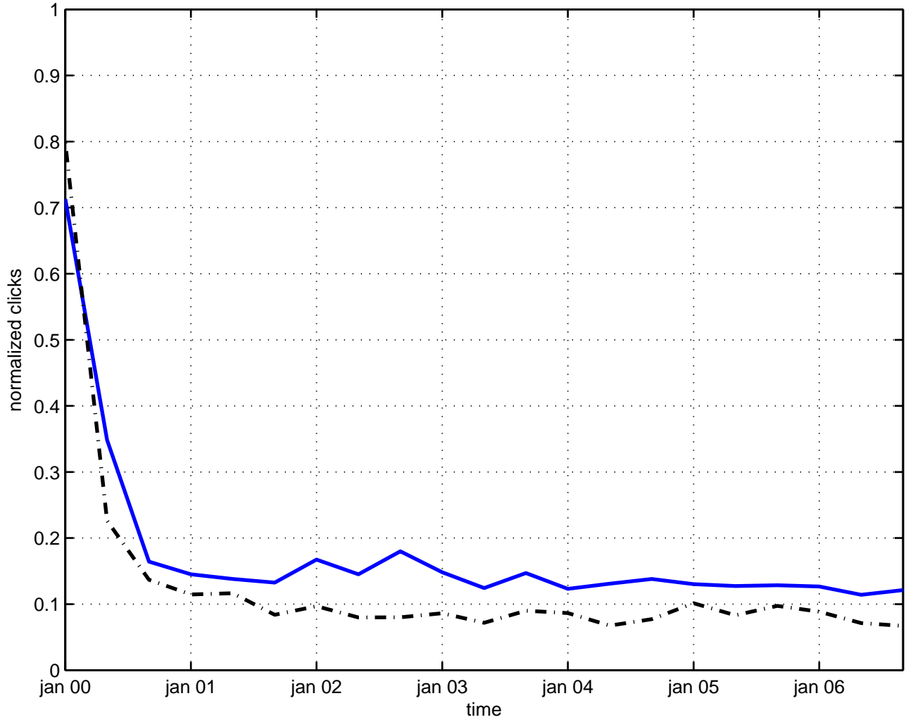
phase space quantum gravity
