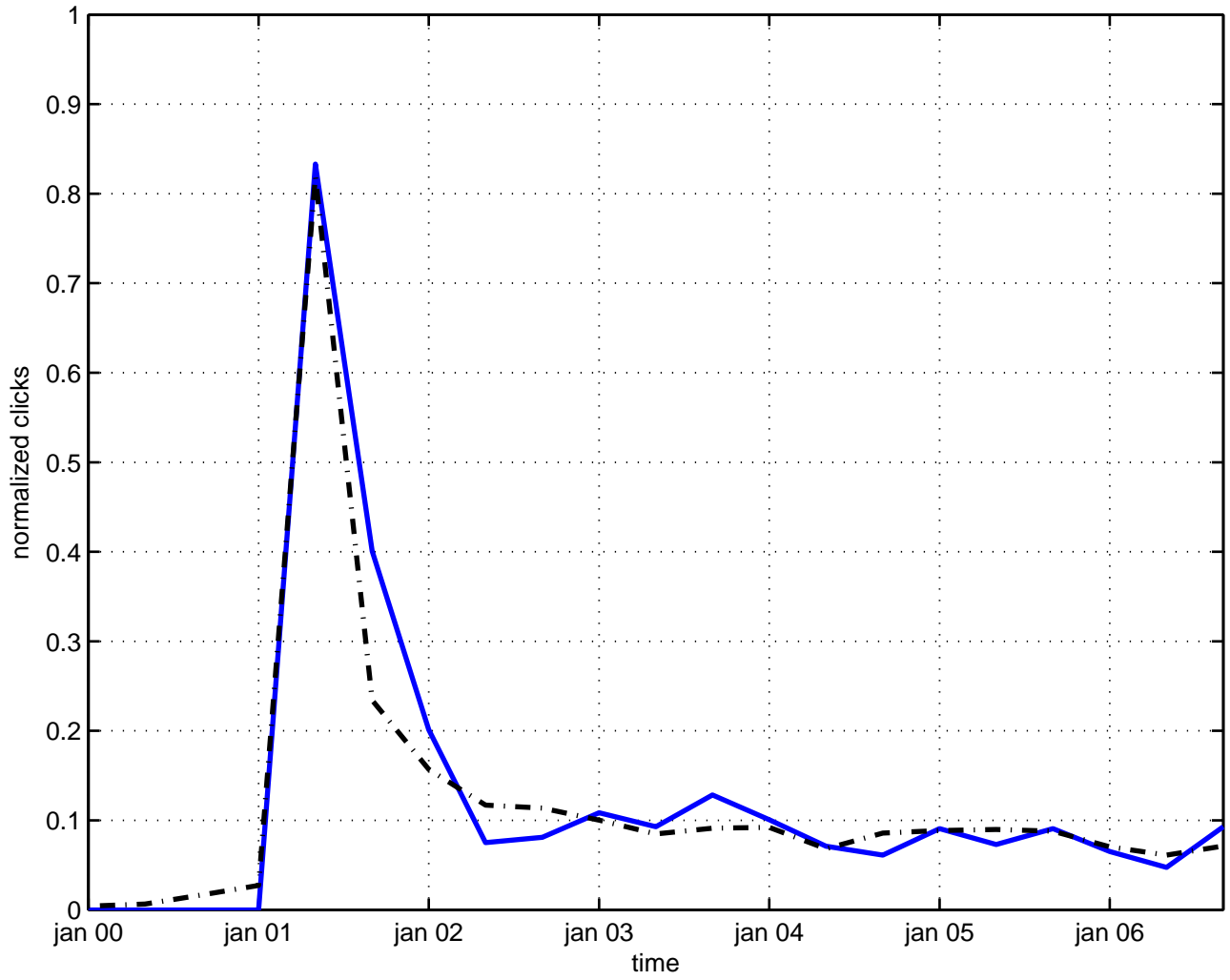
phase space quantization
