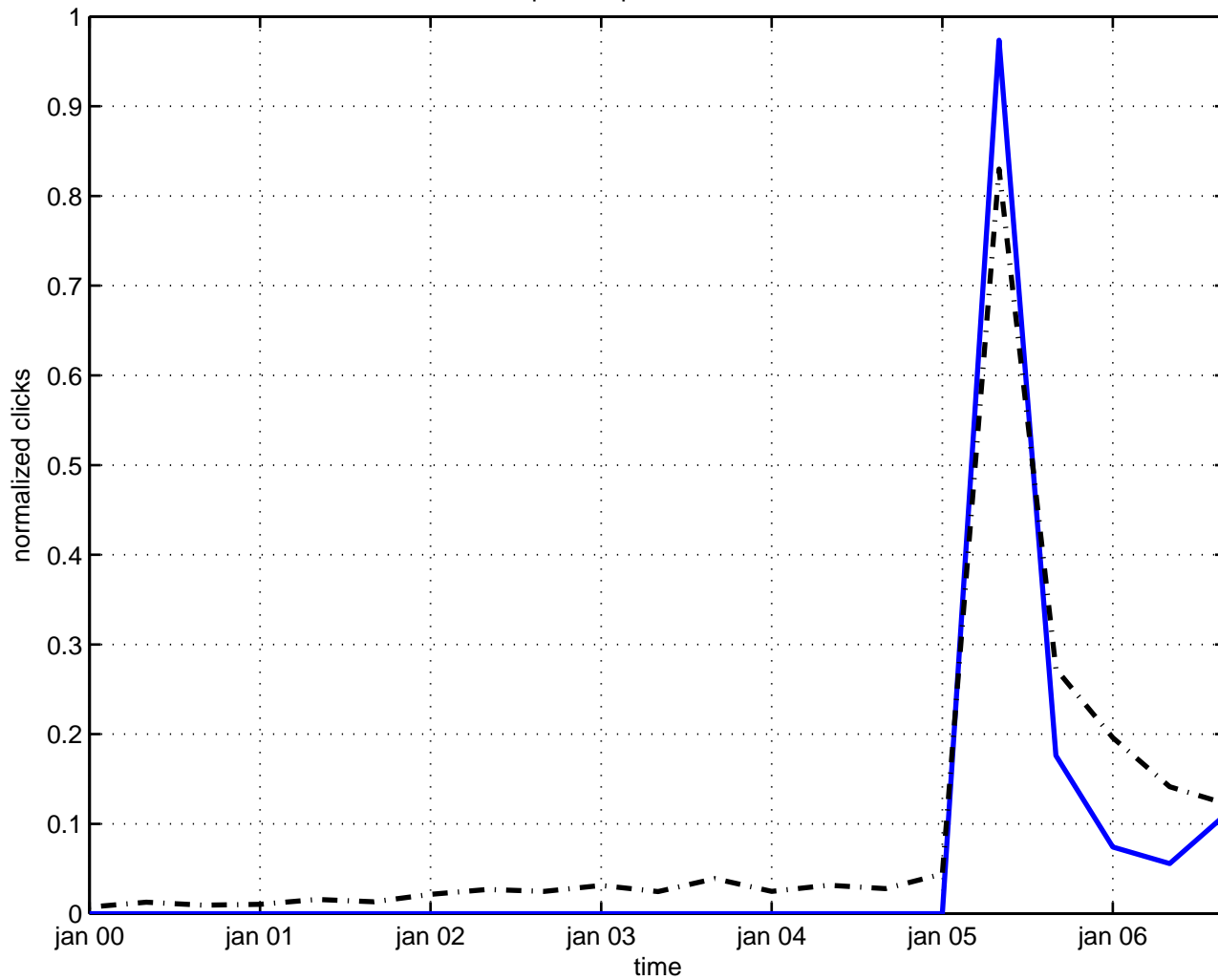
phase space oscillator
