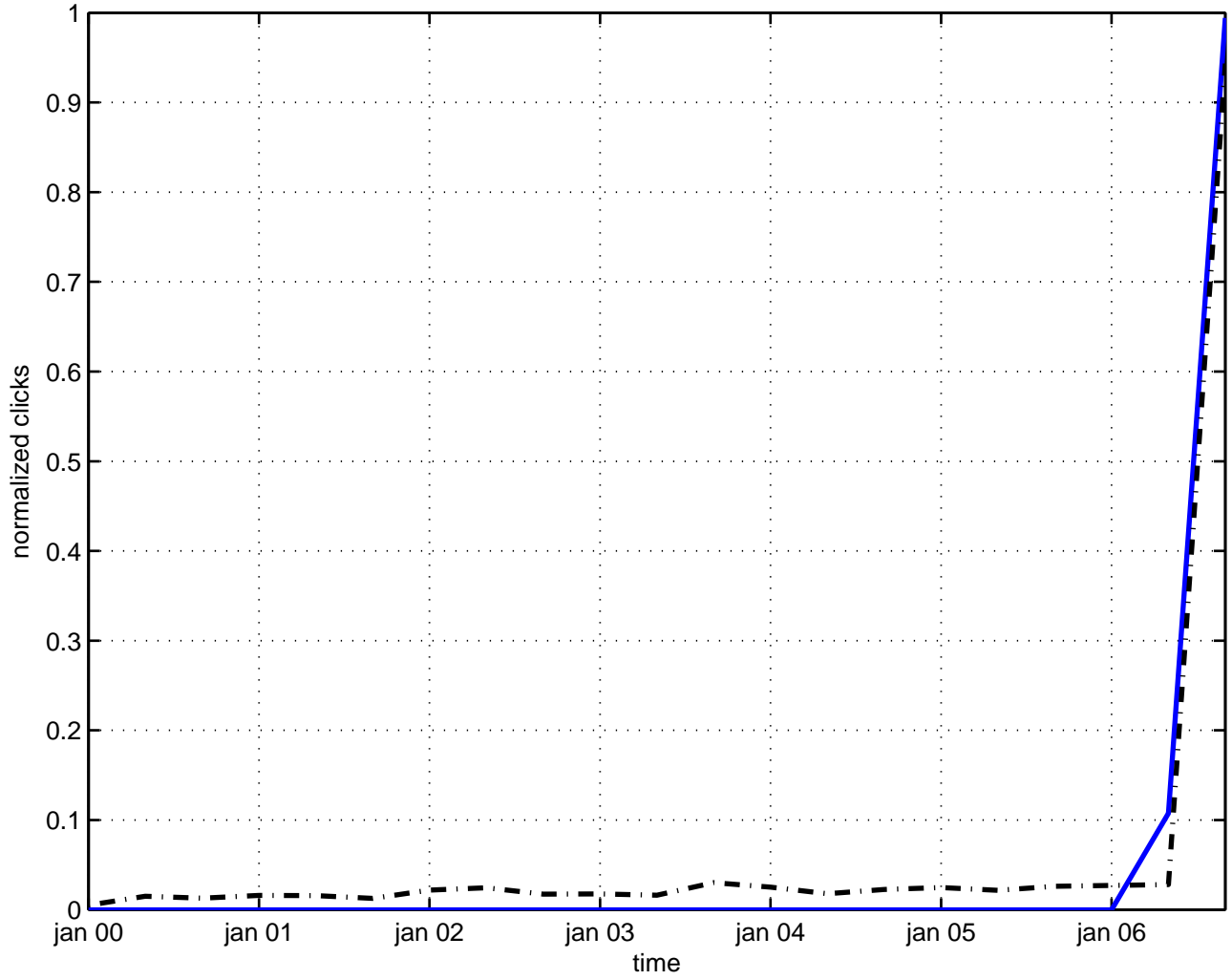
phase space boundary condition
