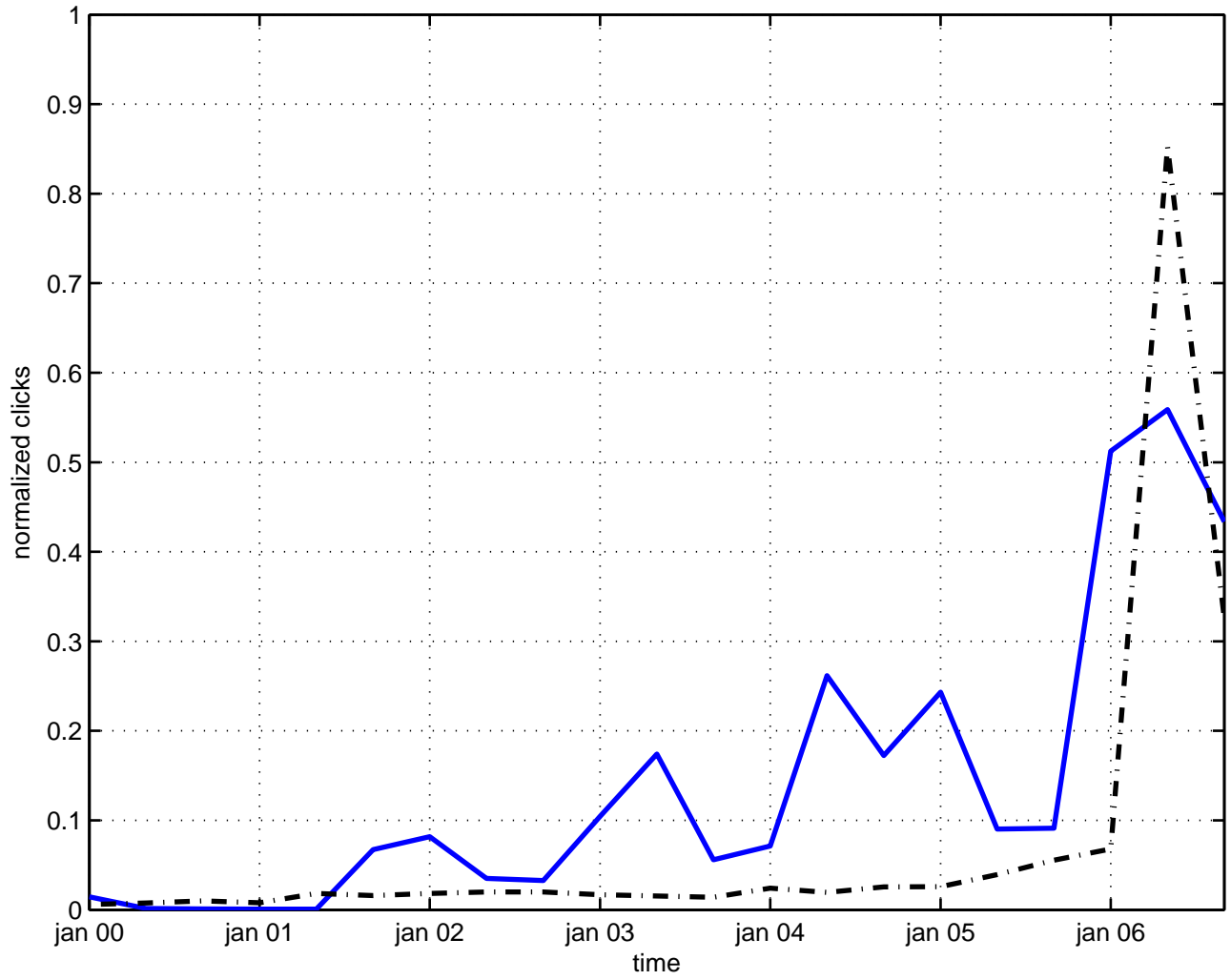
perturbation
