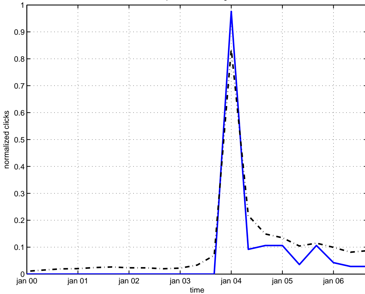
perturbation string
