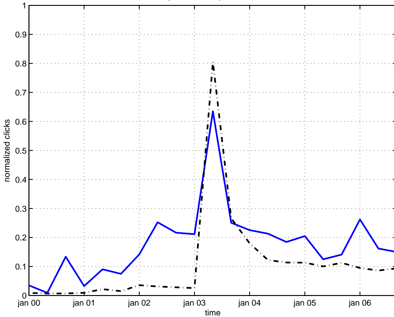
perturbation space-time
