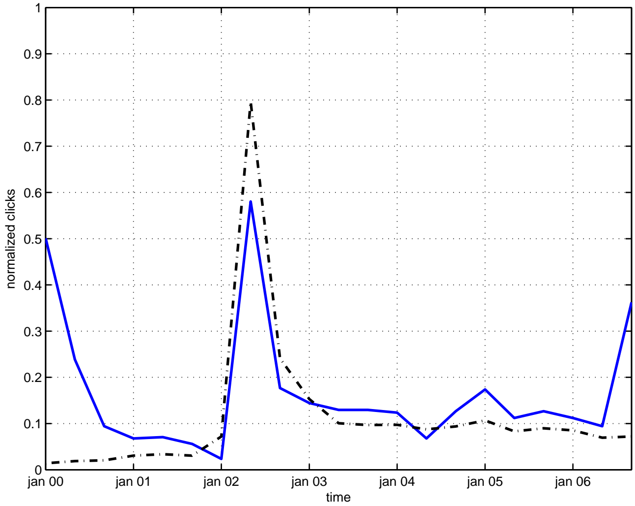
perturbation matter
