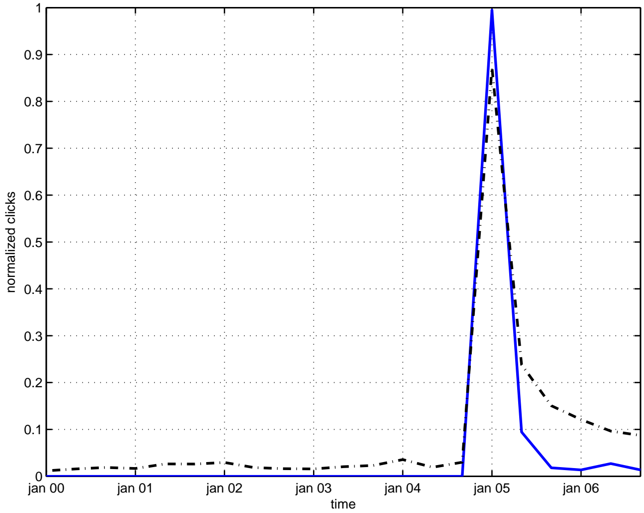
perturbation horizon
