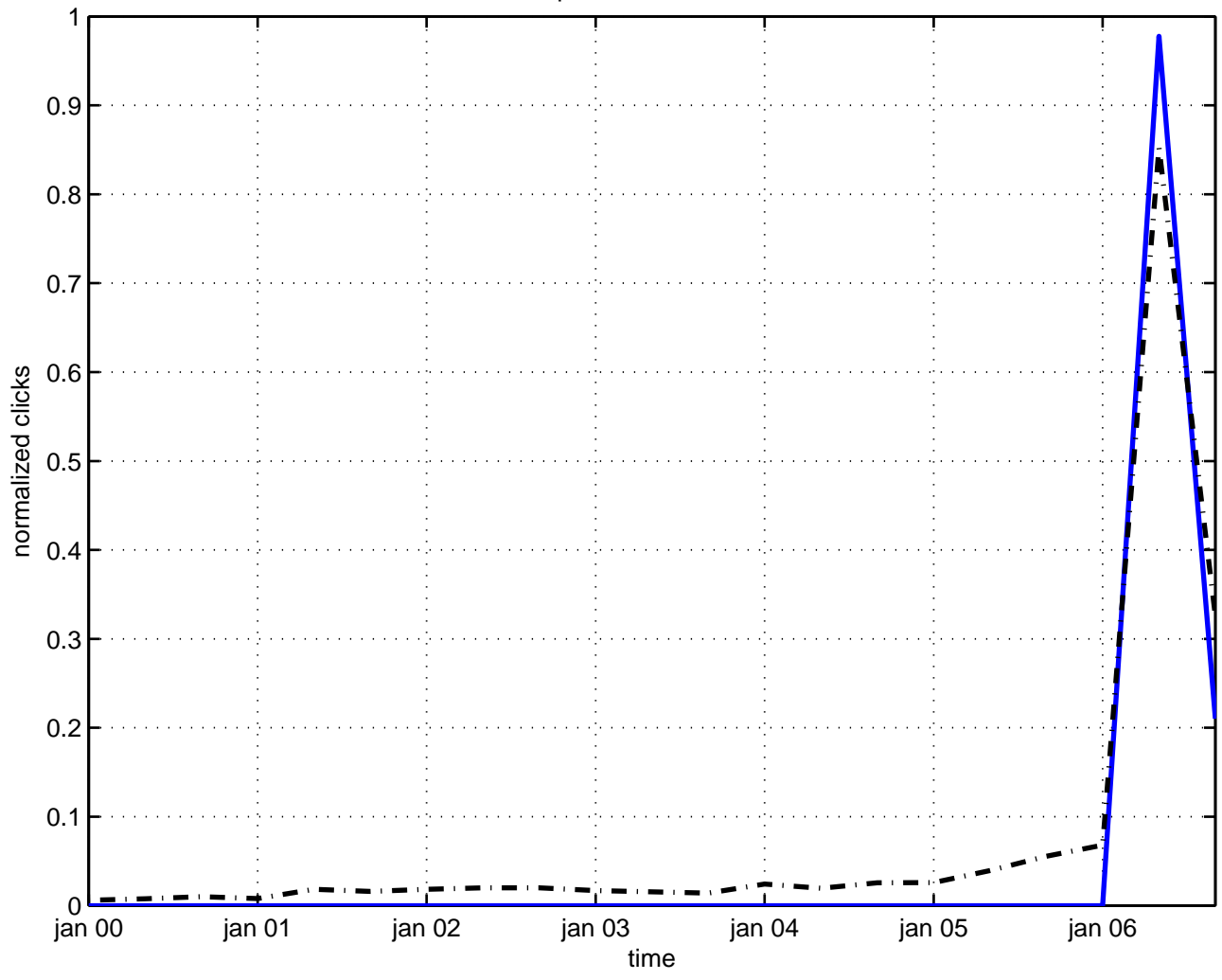
perturbation fluid
