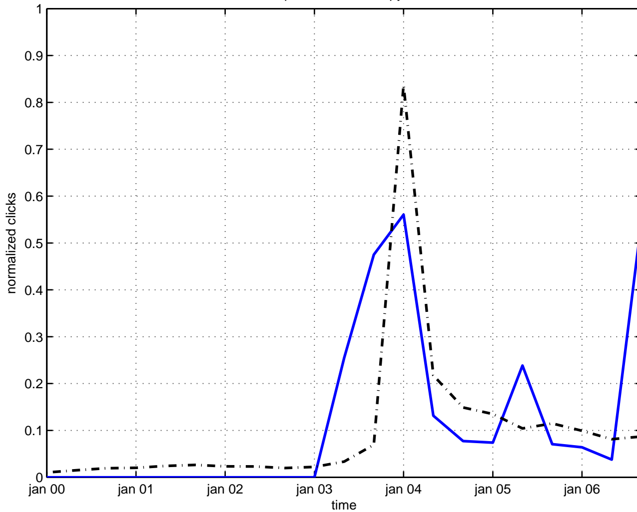
perturbation entropy
