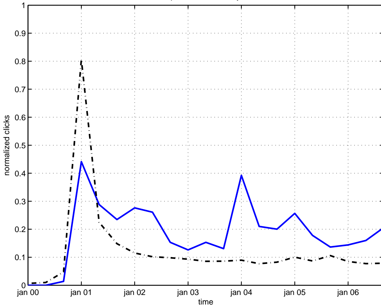
perturbation density
