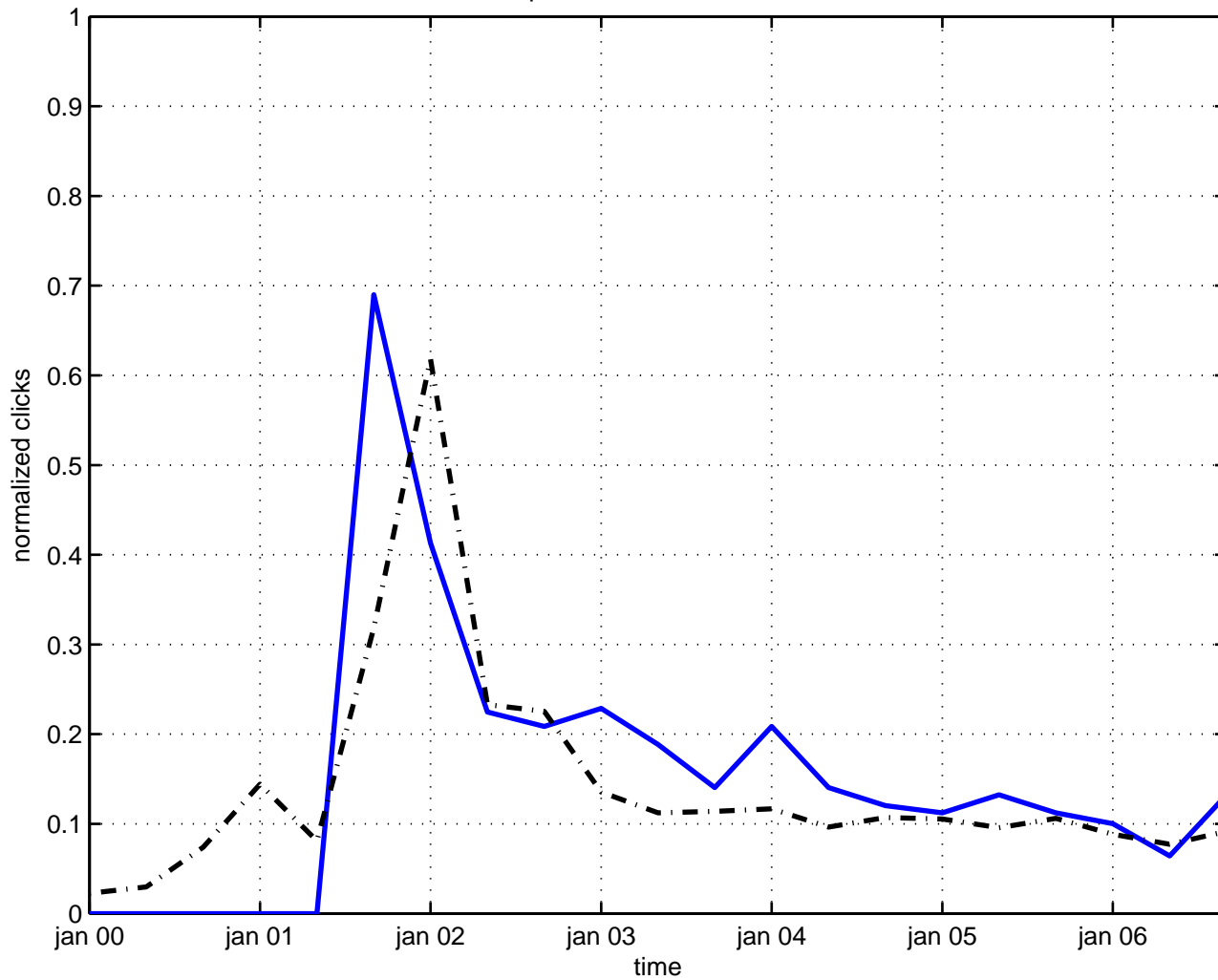
perturbation black hole
