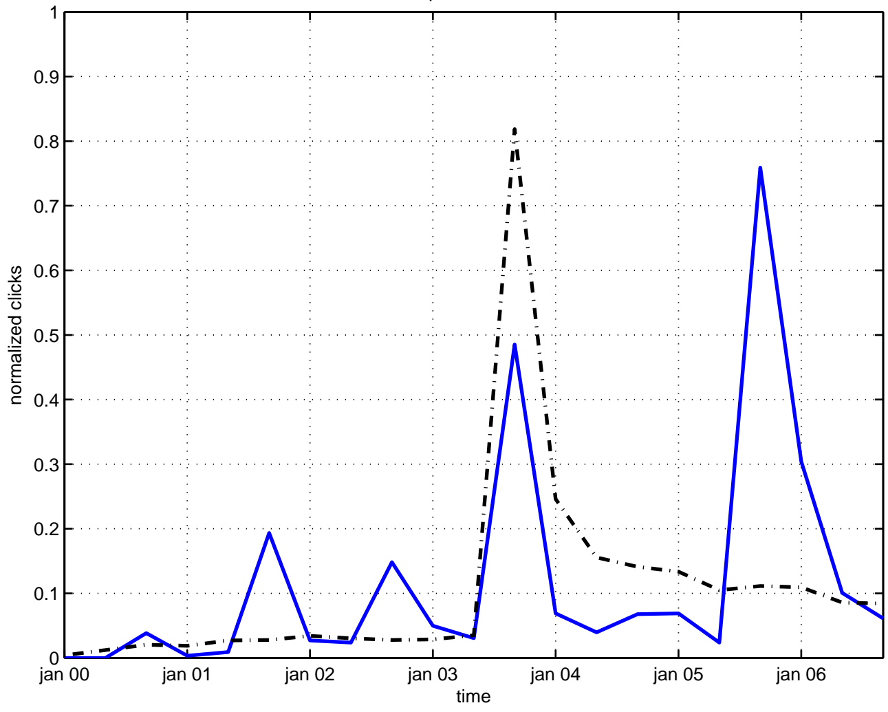
percolation
