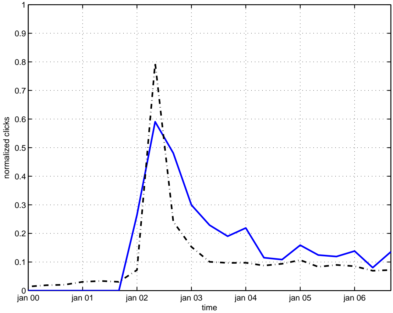
penrose limit
