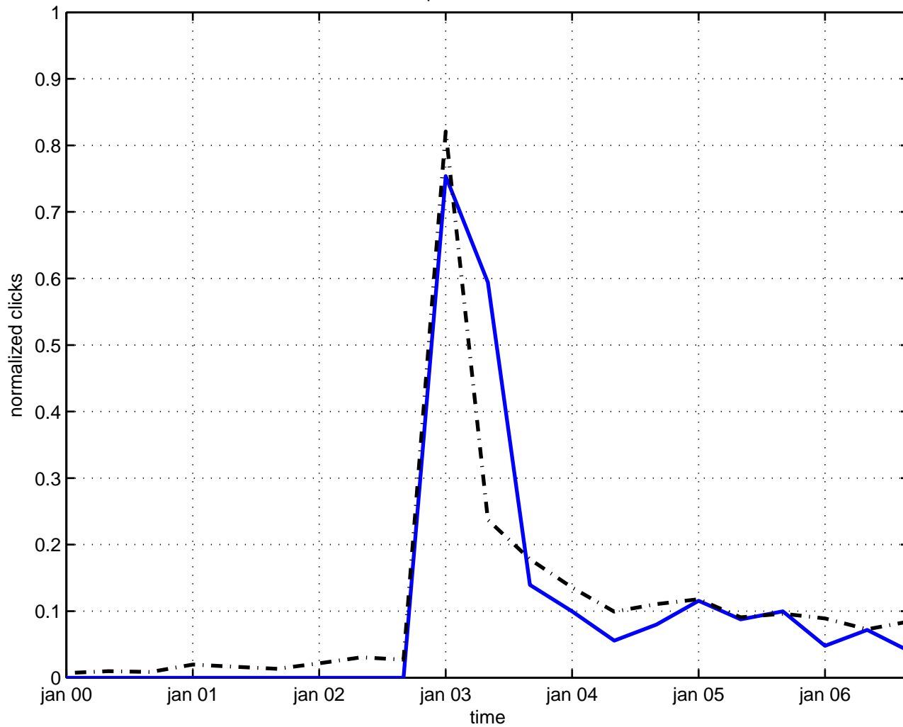
peierls bracket
