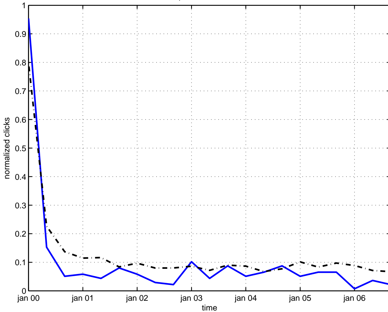
pauli-fierz model
