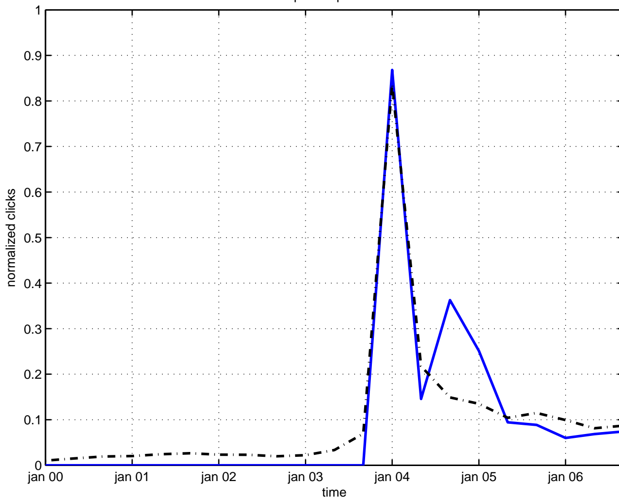
pauli equation
