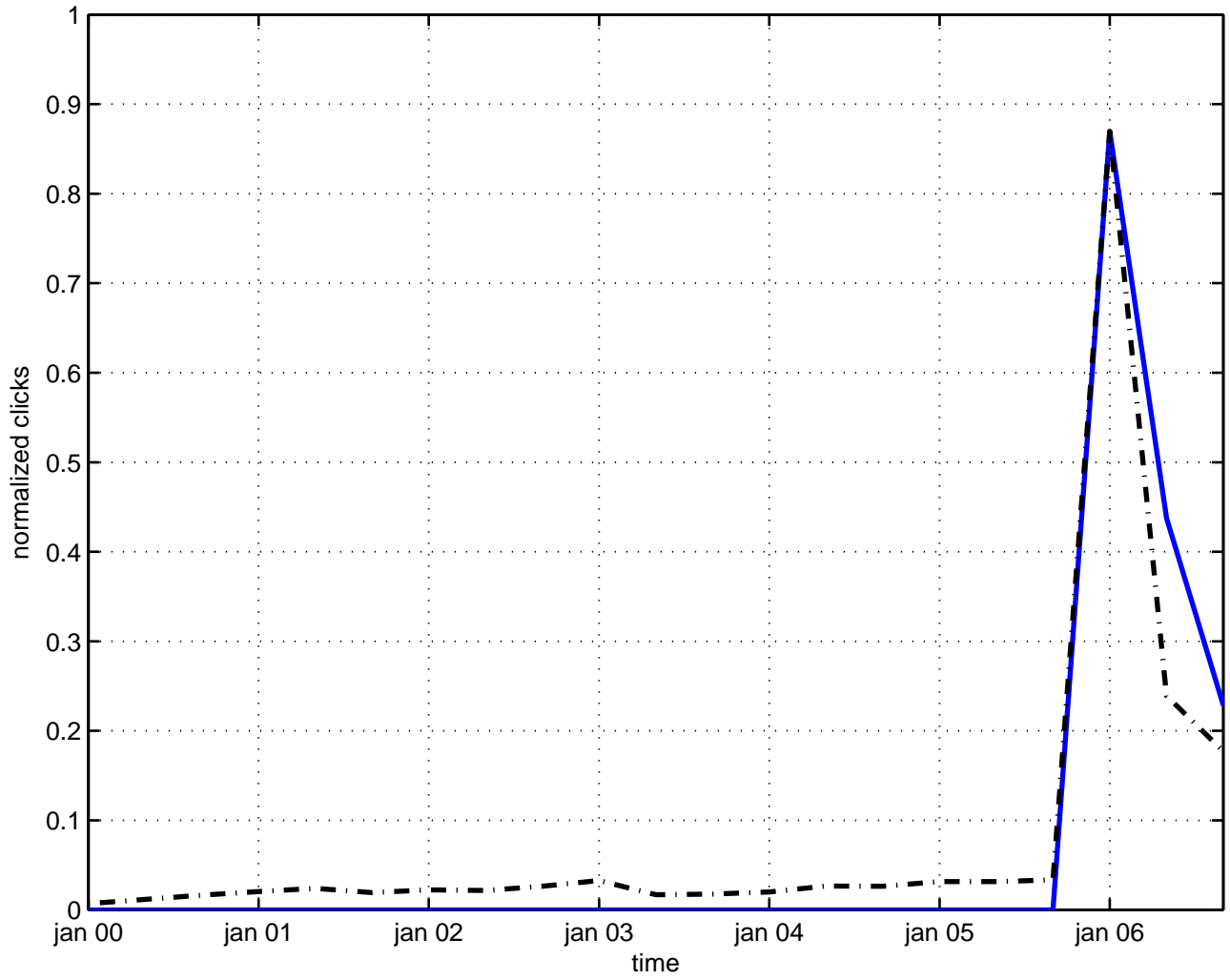
pati-salam model
