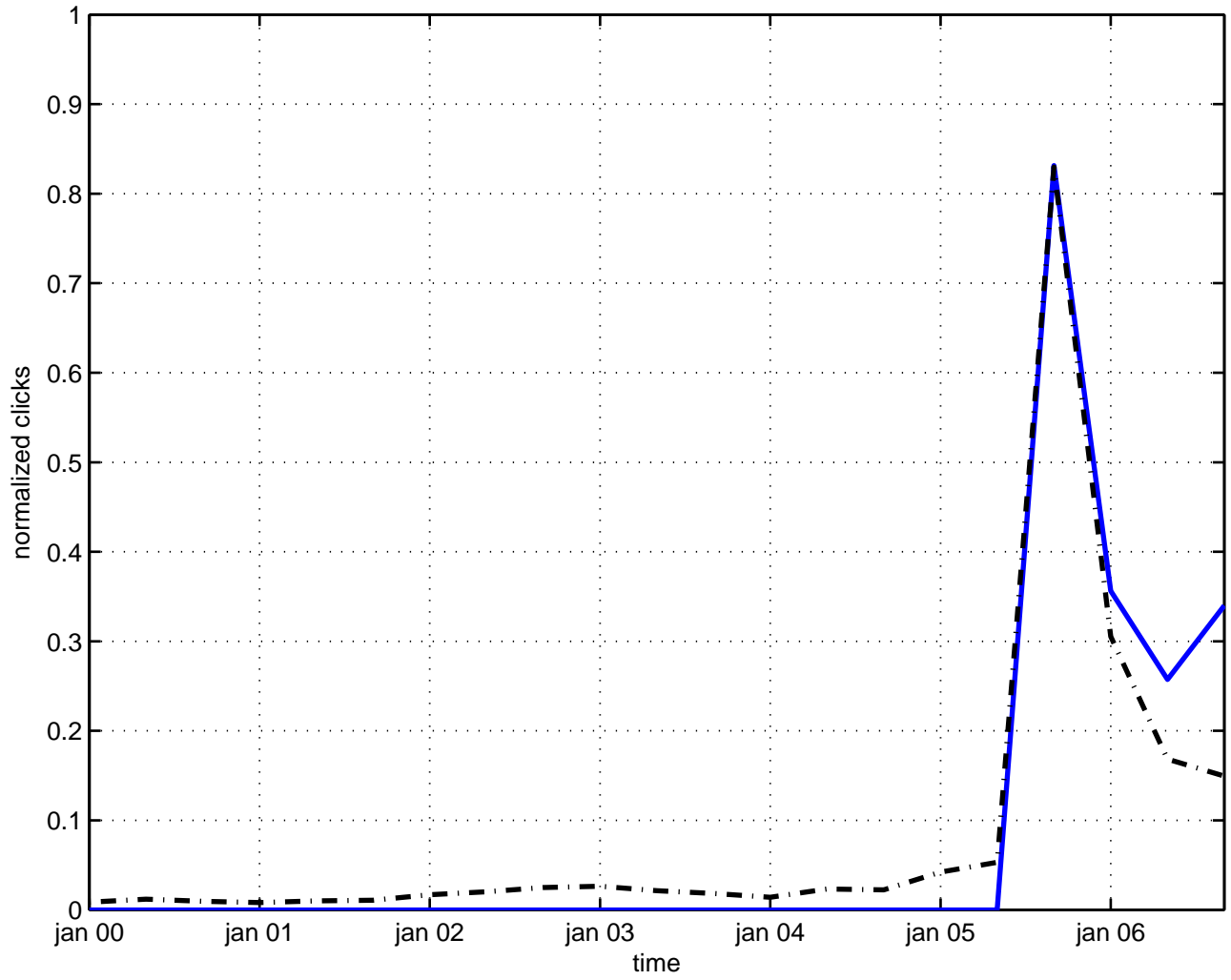
parton multiple production
