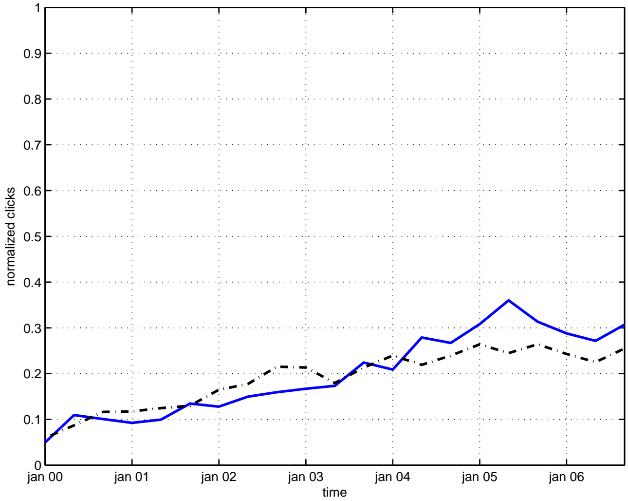
partition function
