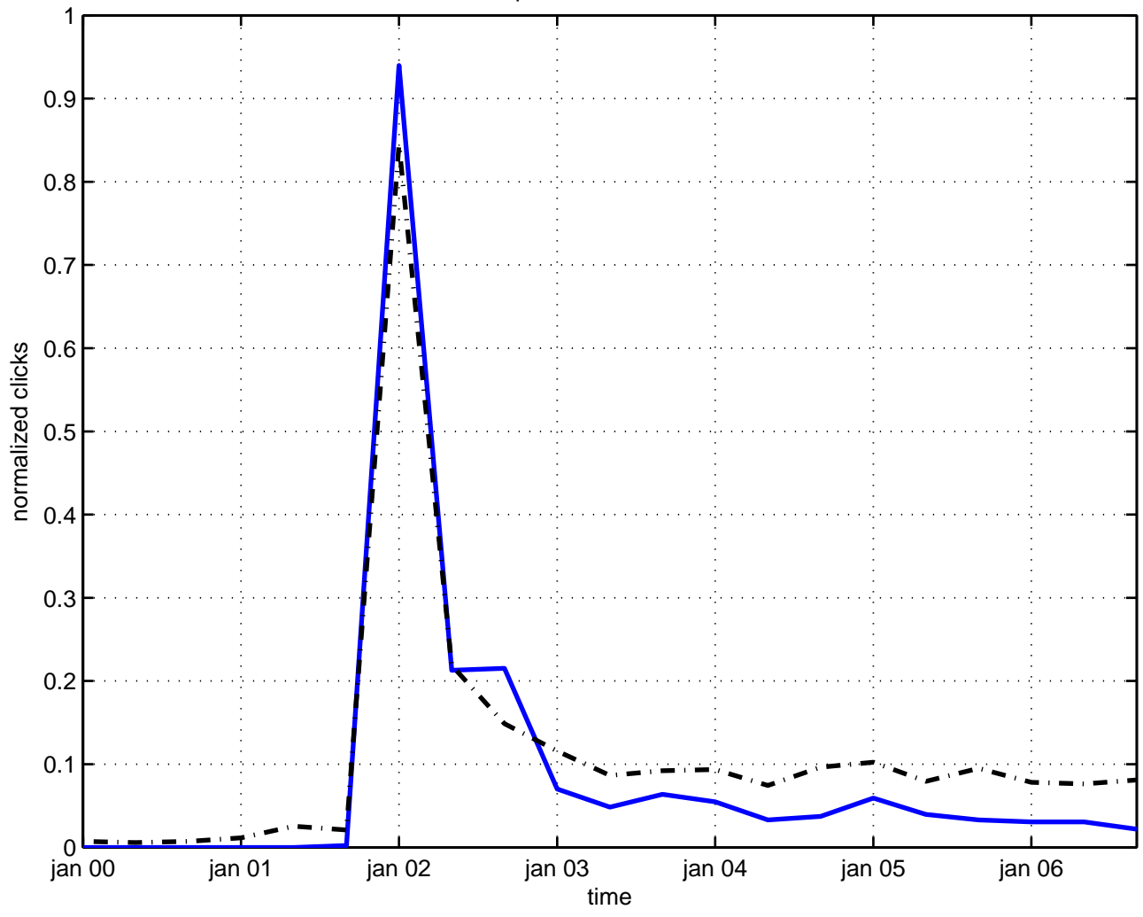
particle black hole
