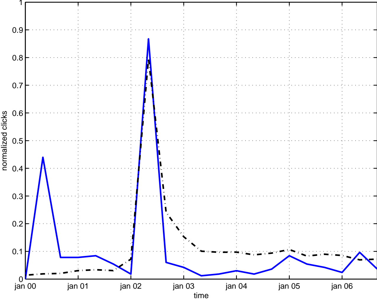
parity higgs particle
